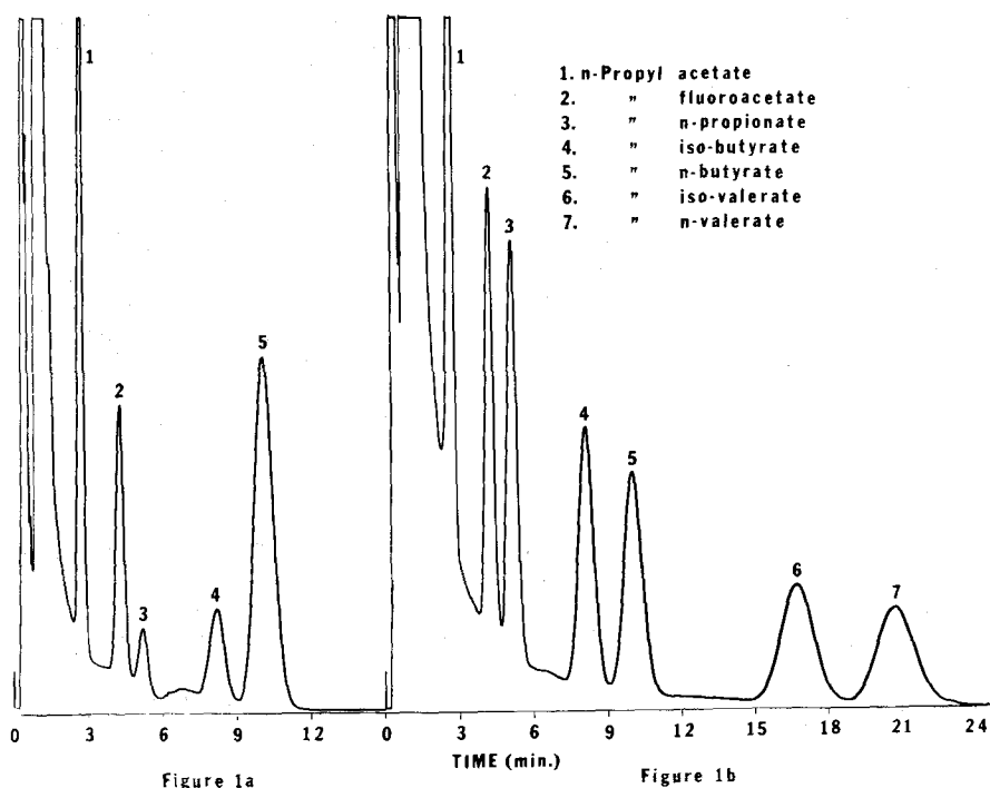
Fig. 1a. Gas chromatogram of a sample of dog stomach contents spiked with the equivalent of 10 ppm of 1080.
